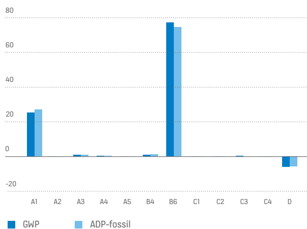
Figure 1. Results for GWP and ADP of fossil resources of KONE 3000S MonoSpace® elevator
